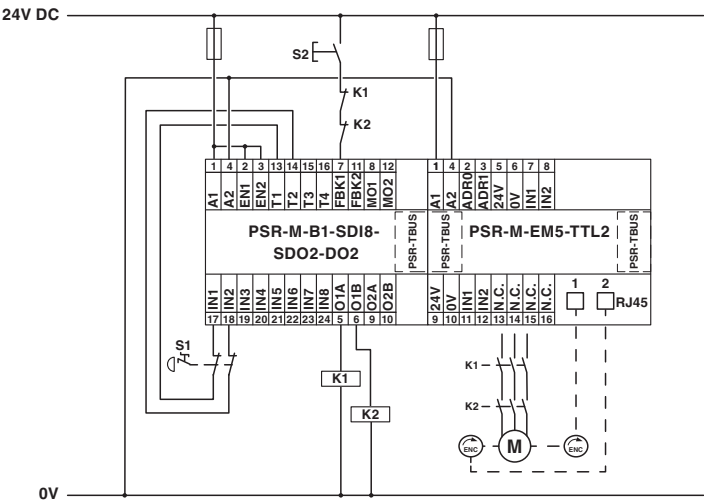
Application drawing
